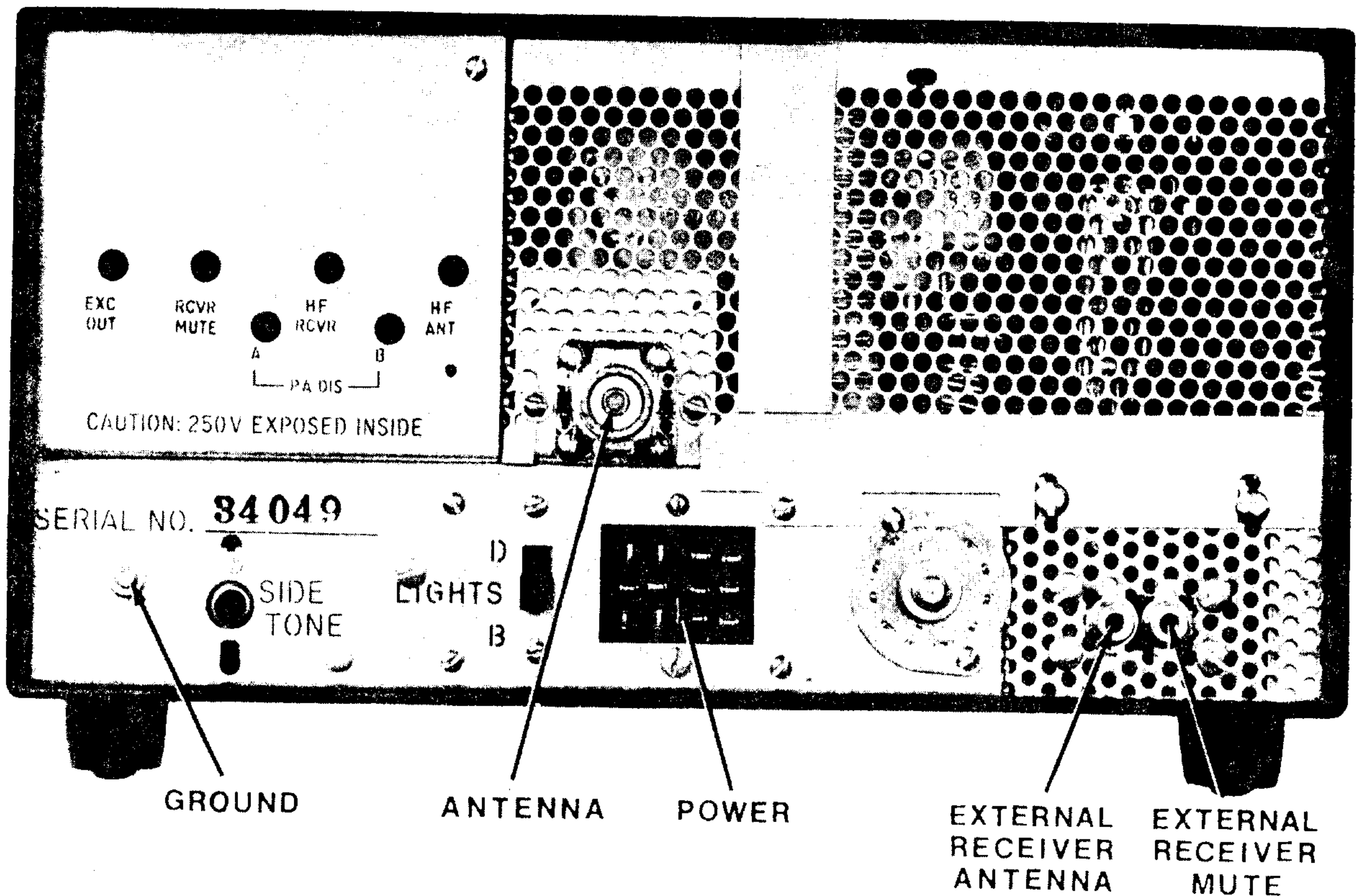
Figure 2-2. Rear Chassis Connectors
