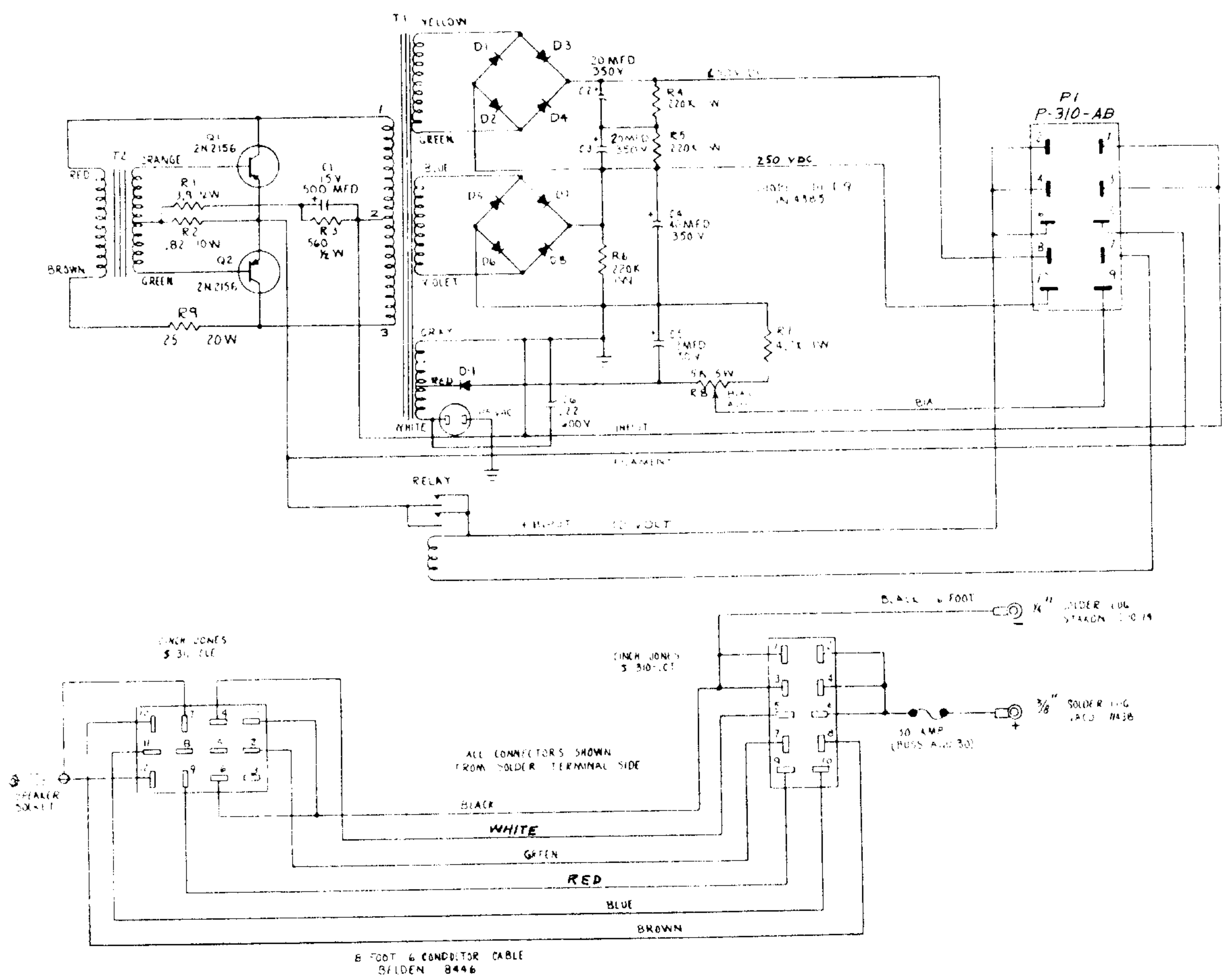
Figure 5-4. DC-4 Power Supply Schematic
