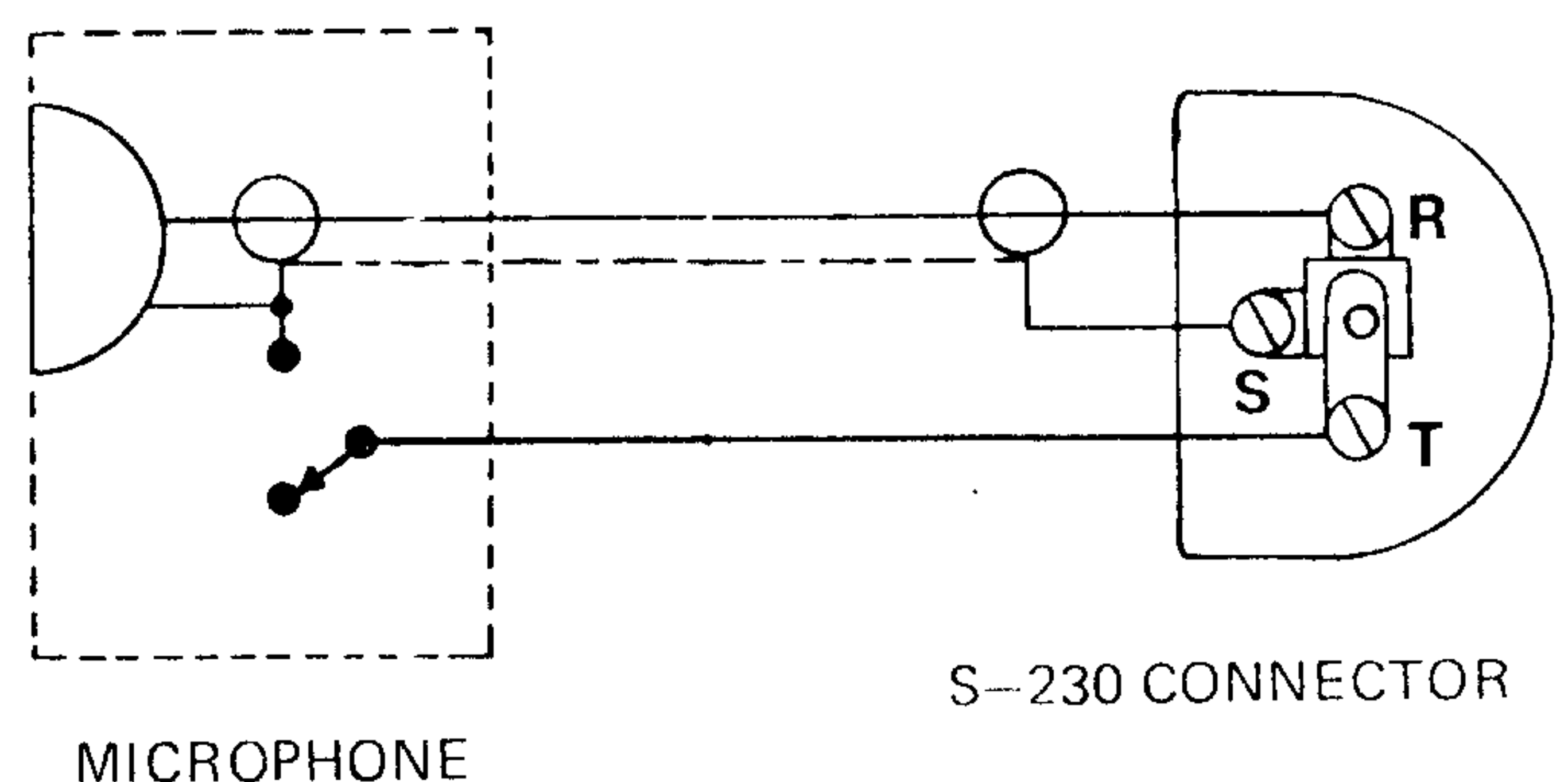
Figure 2-1. Microphone Connections
