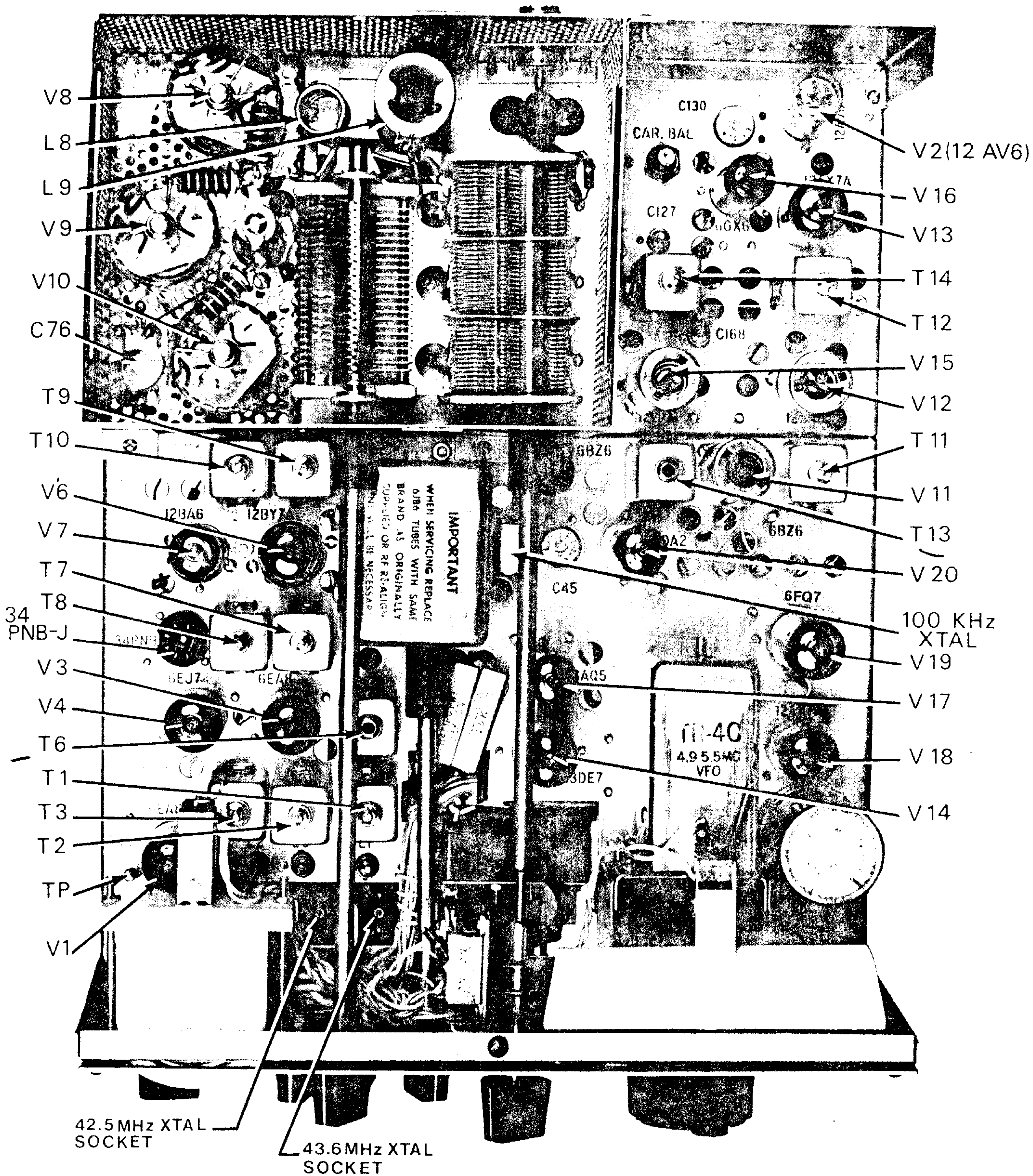
Figure 5-1. Alignment Locations, Top View
